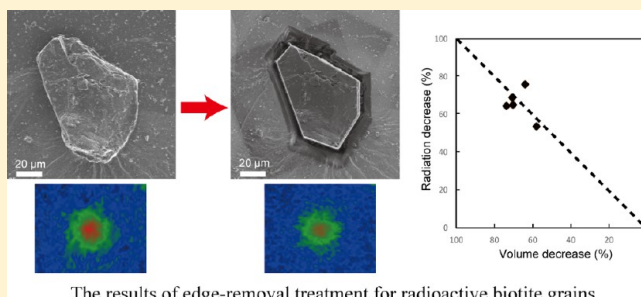
The results of edge-removal treatment for radioactive biotite grains
